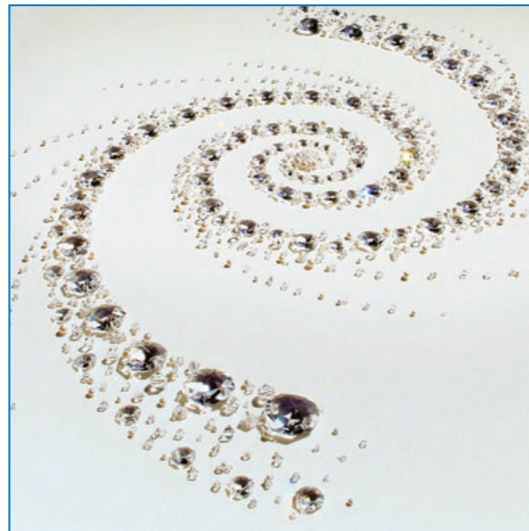
Whirlpool Galaxy 40" x 40"
